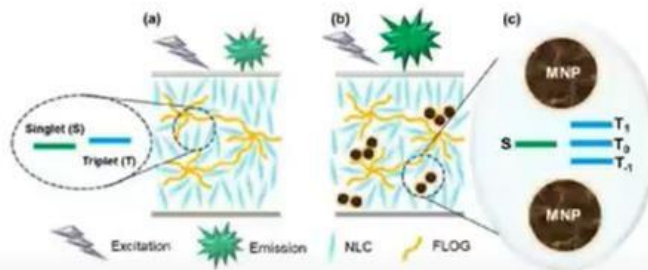
Figure: Schematic representation of the emission process in the (a), (b) FNL C-MNP mixtures filled in a liquid crystal test cell; (c) depicts the magnetic field effect (MFE) on the excitonic states leading to enhancement of PL intensity in the FNL C-MNP system.
